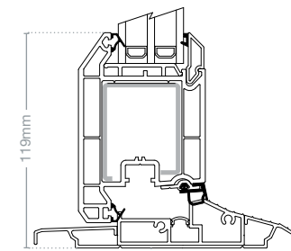
Low threshold assembly EWS 7545A and EWS 7546A
