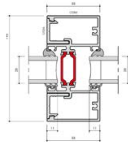
Screen Mullion
