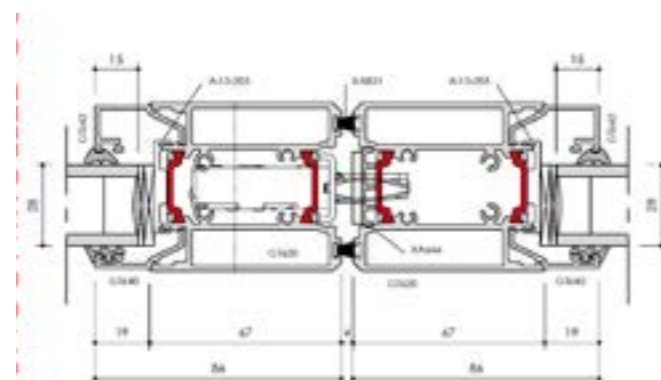
Meeting Stile
