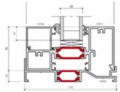
Screen Cill
